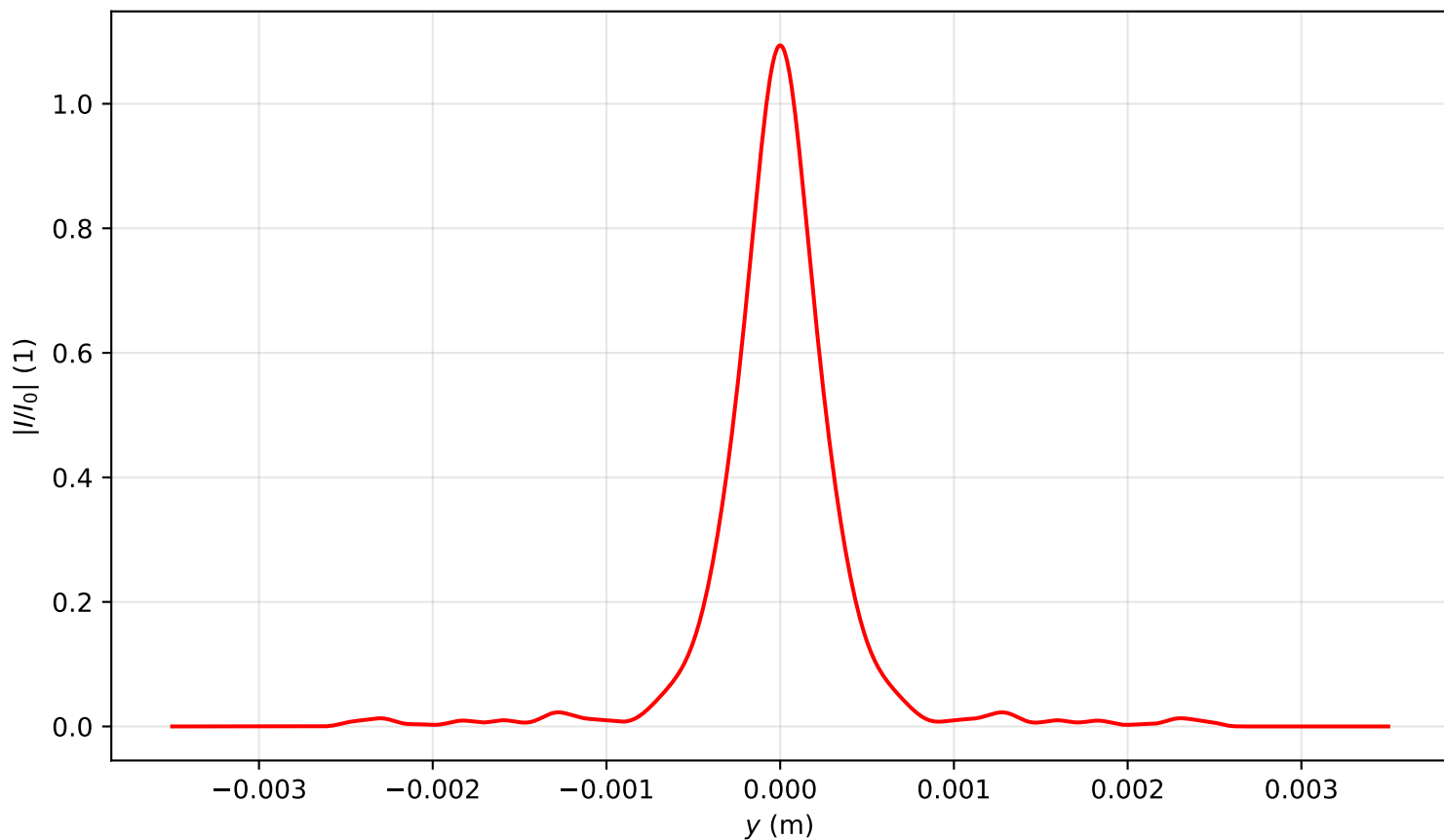
Intensity profile I(x=0, y, z=3.821)/I_0 , \text{Pin}=2.0\text{Pcr} , artificial time
